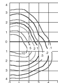
Isofootcandle Lines of Illumination
