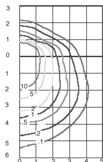
Isofootcandle Lines of Illumination
