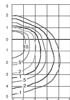
Isofootcandle Lines of Illumination
